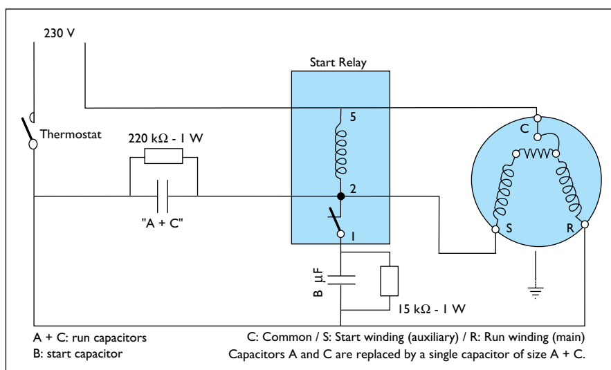
Single phase CSR wiring without trickle circuit
